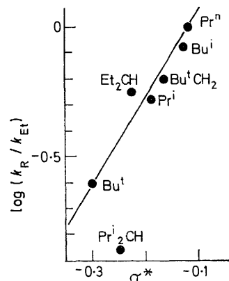
FIGURE 1 Competition experiments. Reaction of EtMgBr with acid chlorides, CuCl catalyst ( \rho^* = 2.96 \pm 0.38 , r_d^2 = 0.97 )
